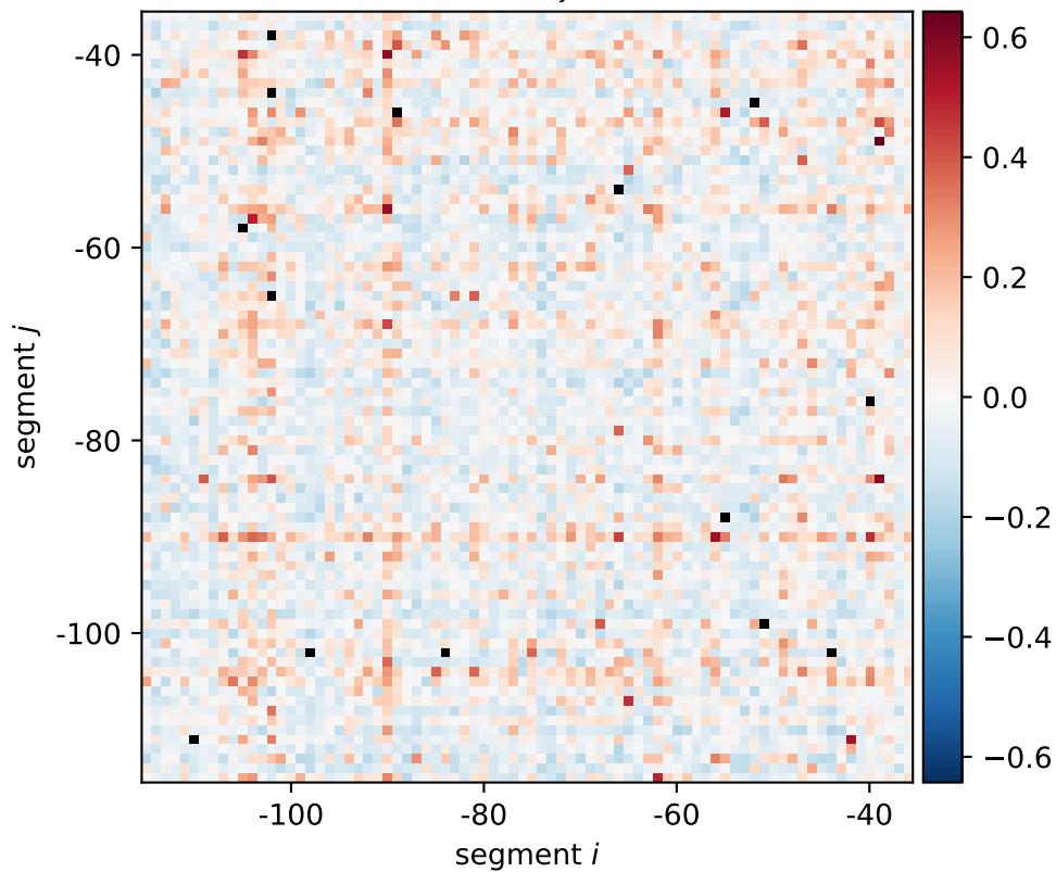
yajL expression shift \xi_{i,j}[0101, 0110, 1010]
