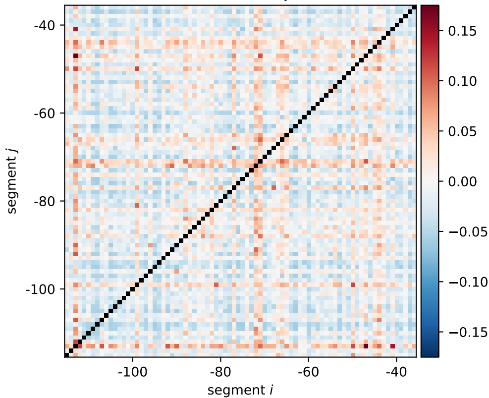
ybdG expression shift \xi_{i,j}[0011, 1100]
