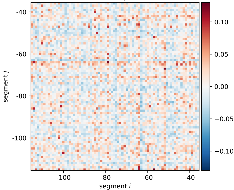
ybdG expression shift \xi_{i,j}[0101, 0110, 1010]
