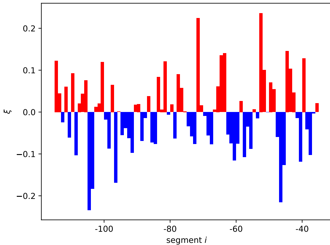
ybdG expression shift \xi_i[11]
