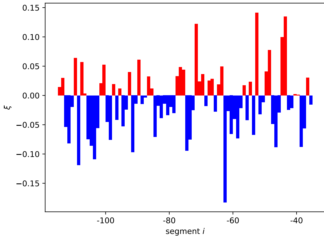
ybdG expression shift \xi_i[11]
