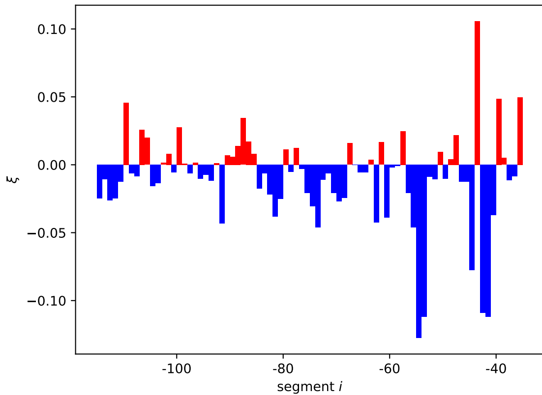
ybeZ expression shift \xi_i[01, 10]
