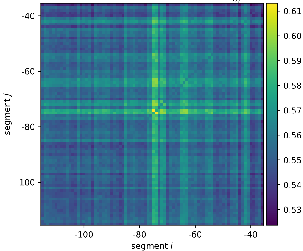
ybeZ mean wildtype expression \mu_{i,j}^*
