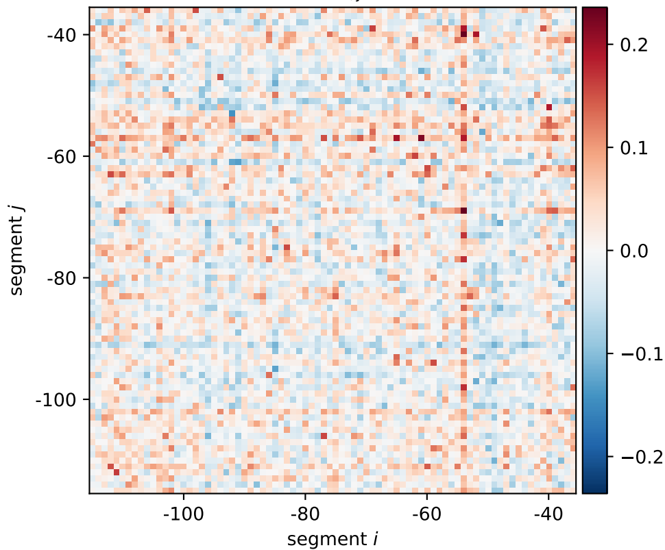
ybiO expression shift \xi_{i,j}[0101, 0110, 1010]
