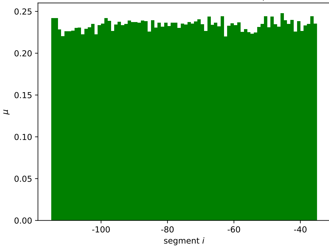
ybiO mean wildtype expression \mu_i^*
