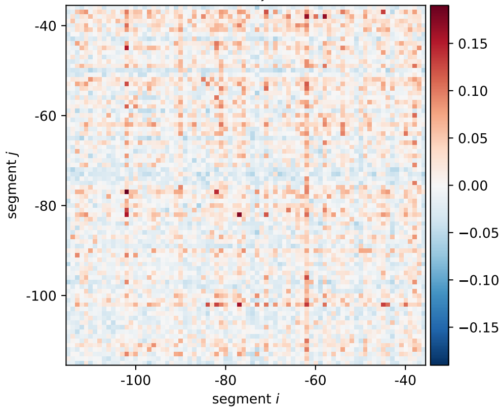
ybiP expression shift \xi_{i,j}[0101, 0110, 1010]
