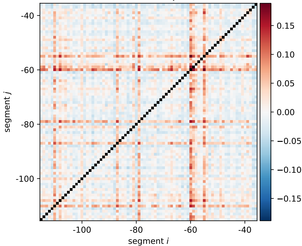
ybiP expression shift \xi_{i,j}[0011, 1100]
