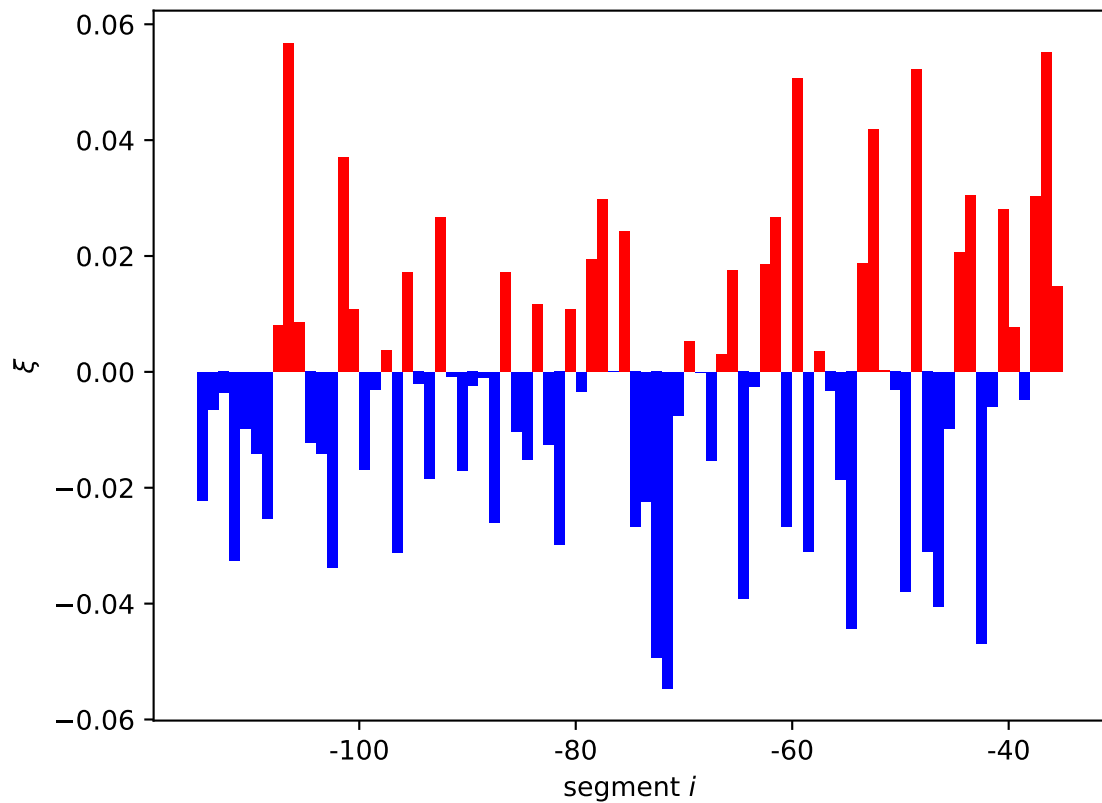
ybiP expression shift \xi_i[01, 10]
