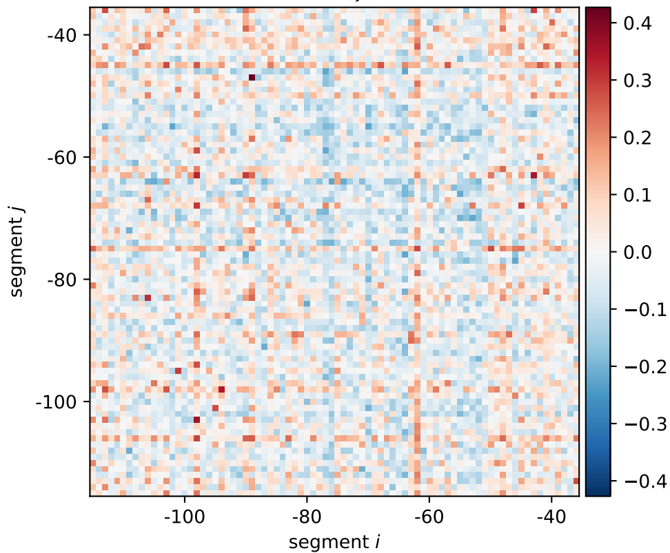
ybjT expression shift \xi_{i,j}[0101, 0110, 1010]
