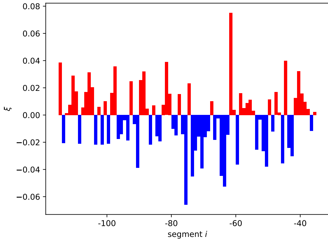
ybjT expression shift \xi_i[01, 10]
