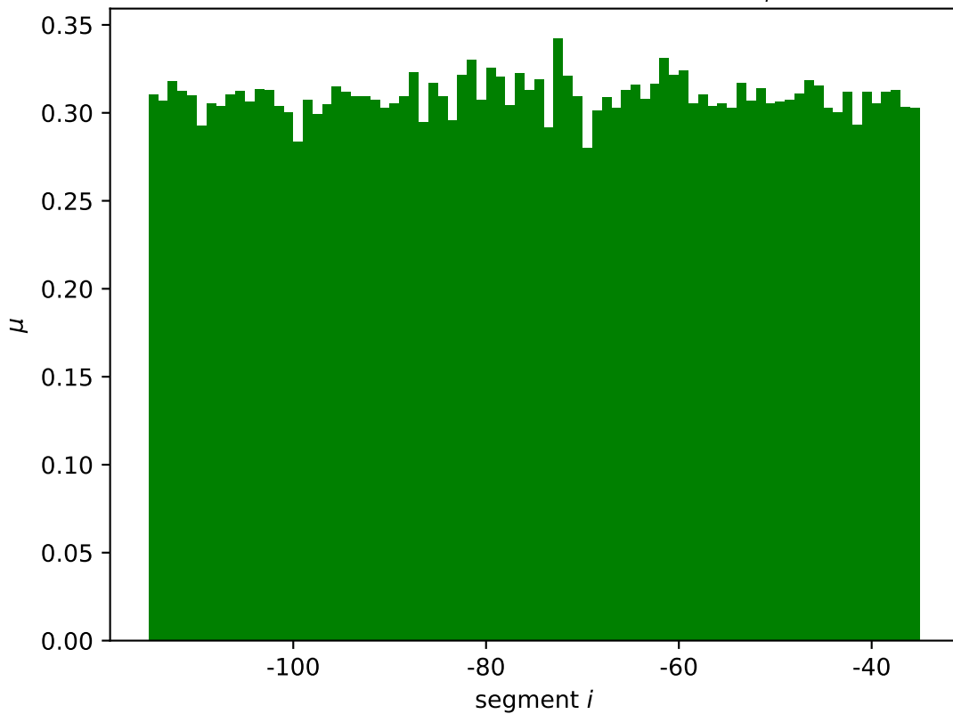
ycbZ mean wildtype expression \mu_i^*
