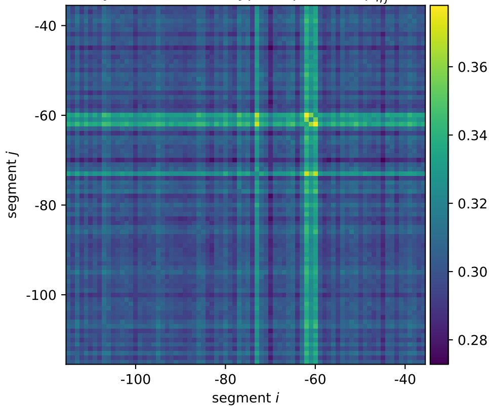
ycbZ mean wildtype expression \mu_{i,j}^*
