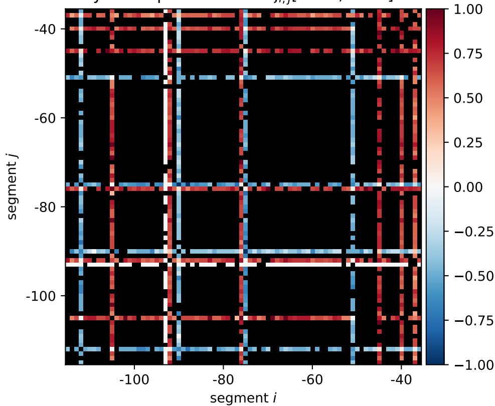
ycbZ expression shift \xi_{i,j}[\text{0011}, \text{1100}]
