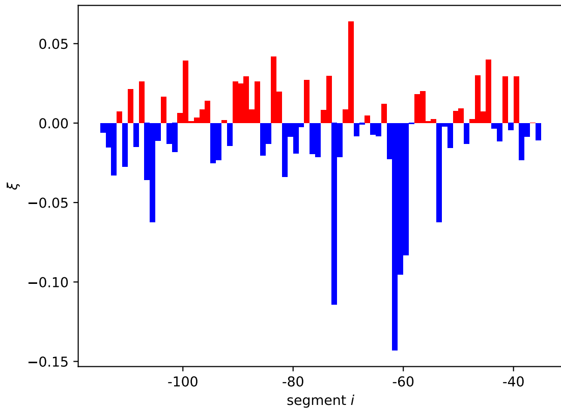
ycbZ expression shift \xi_i[01, 10]
