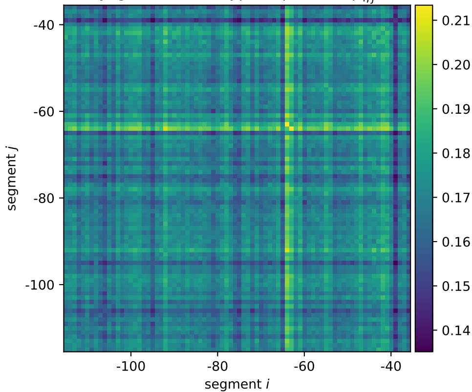
ycgB mean wildtype expression \mu_{i,j}^*
