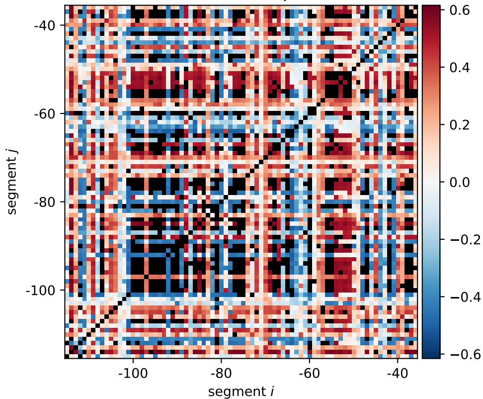
ycgB expression shift \xi_{i,j}[\text{0011}, \text{1100}]
