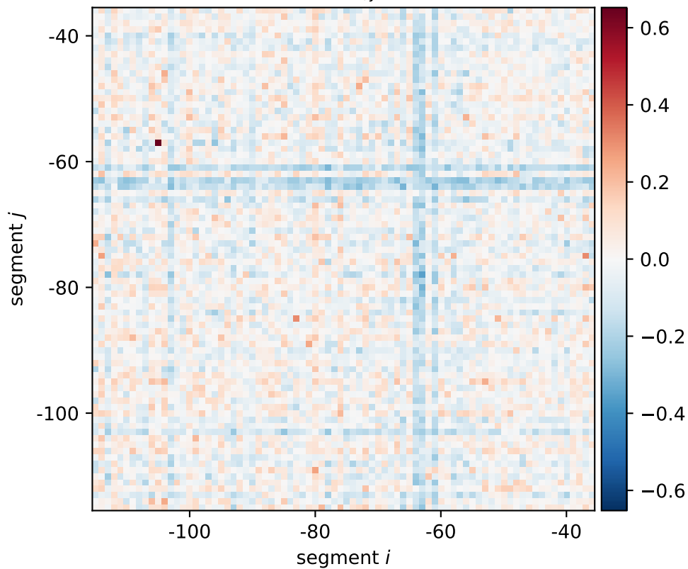
ycgB expression shift \xi_{i,j}[0101, 0110, 1010]
