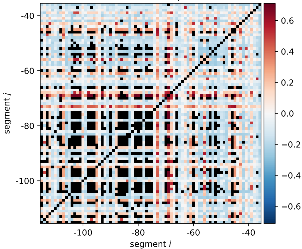
ydho expression shift \xi_{i,j}[0011, 1100]
