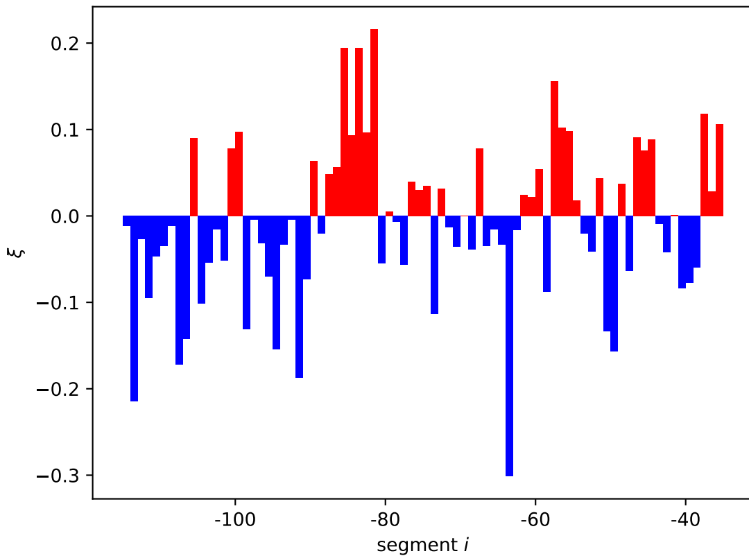
ydho expression shift \xi_i[01, 10]
