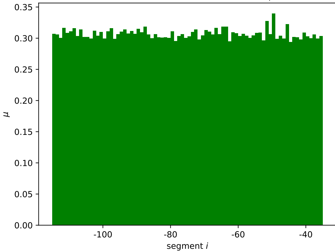
ydhO mean wildtype expression \mu_i^*
