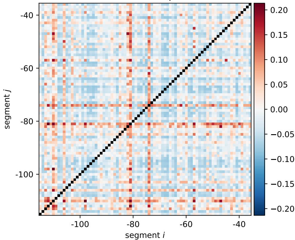
ydjA expression shift \xi_{i,j}[0011, 1100]
