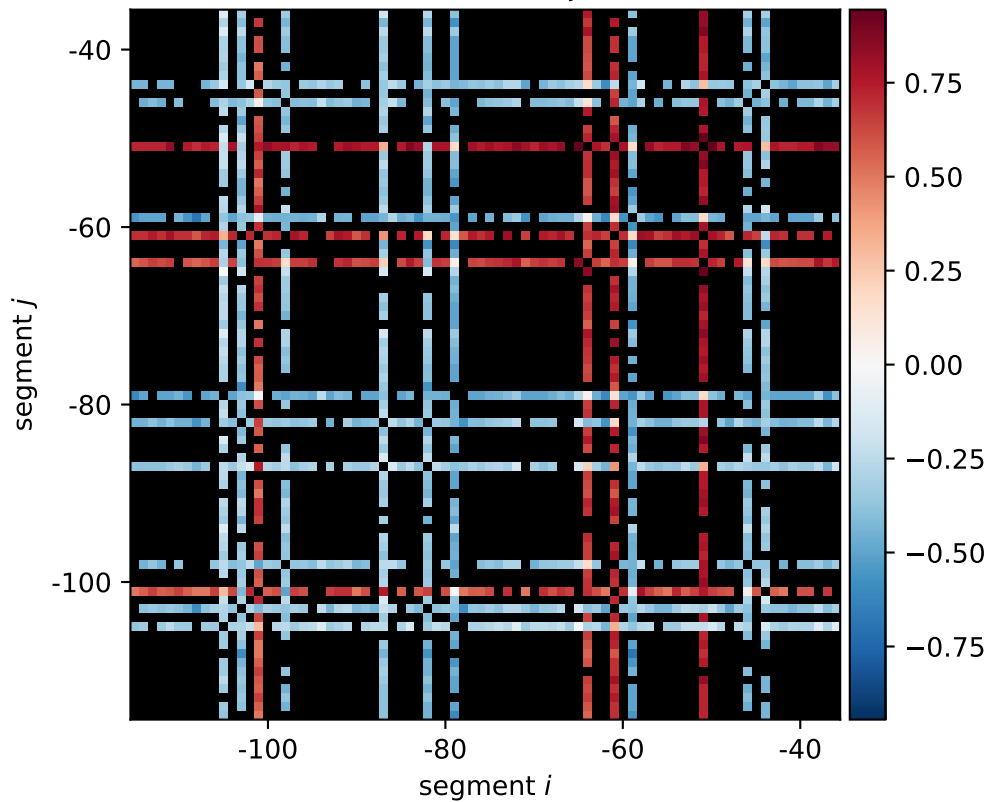
yecE expression shift \xi_{i,j}[0011, 1100]
