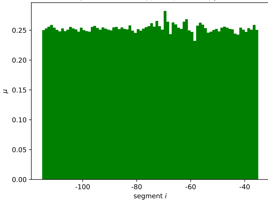
yecE mean wildtype expression \mu_i^*
