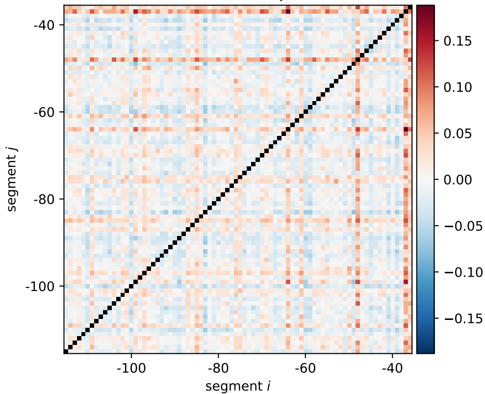
yedK expression shift \xi_{i,j}[0011, 1100]
