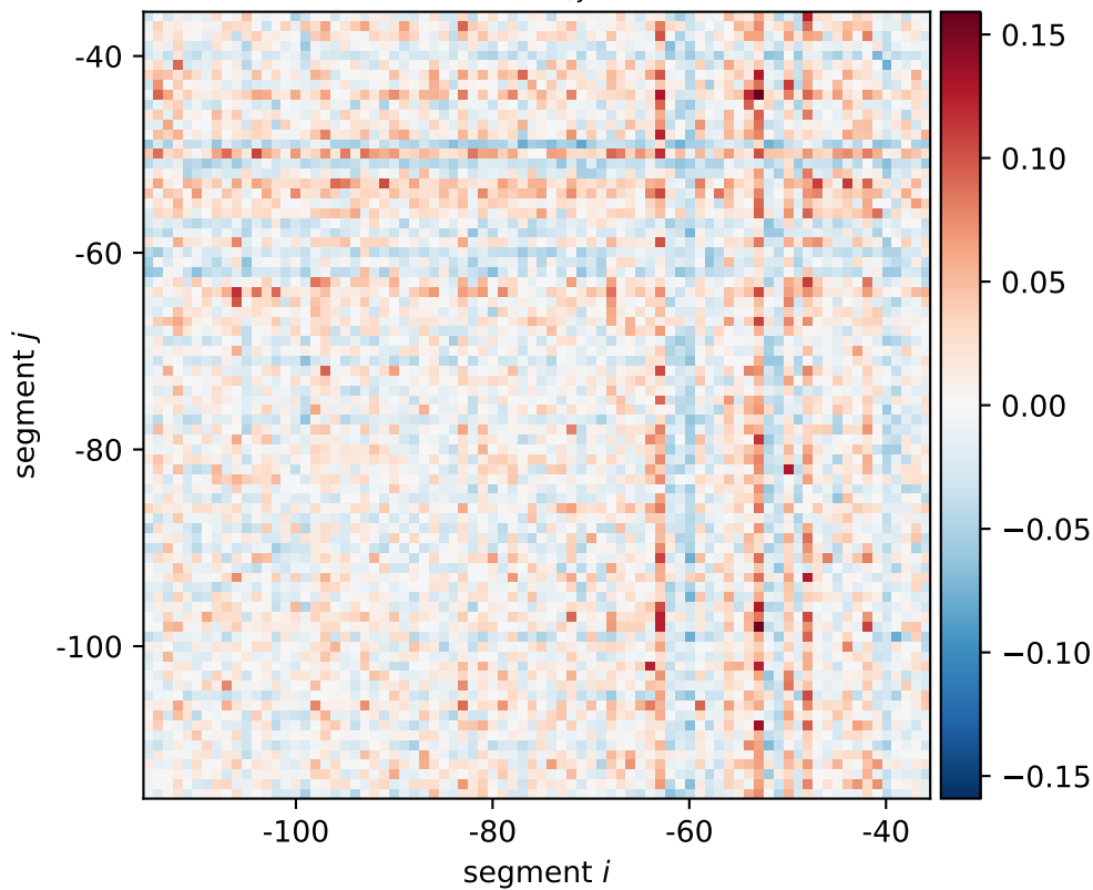
yedK expression shift \xi_{i,j}[0101, 0110, 1010]
