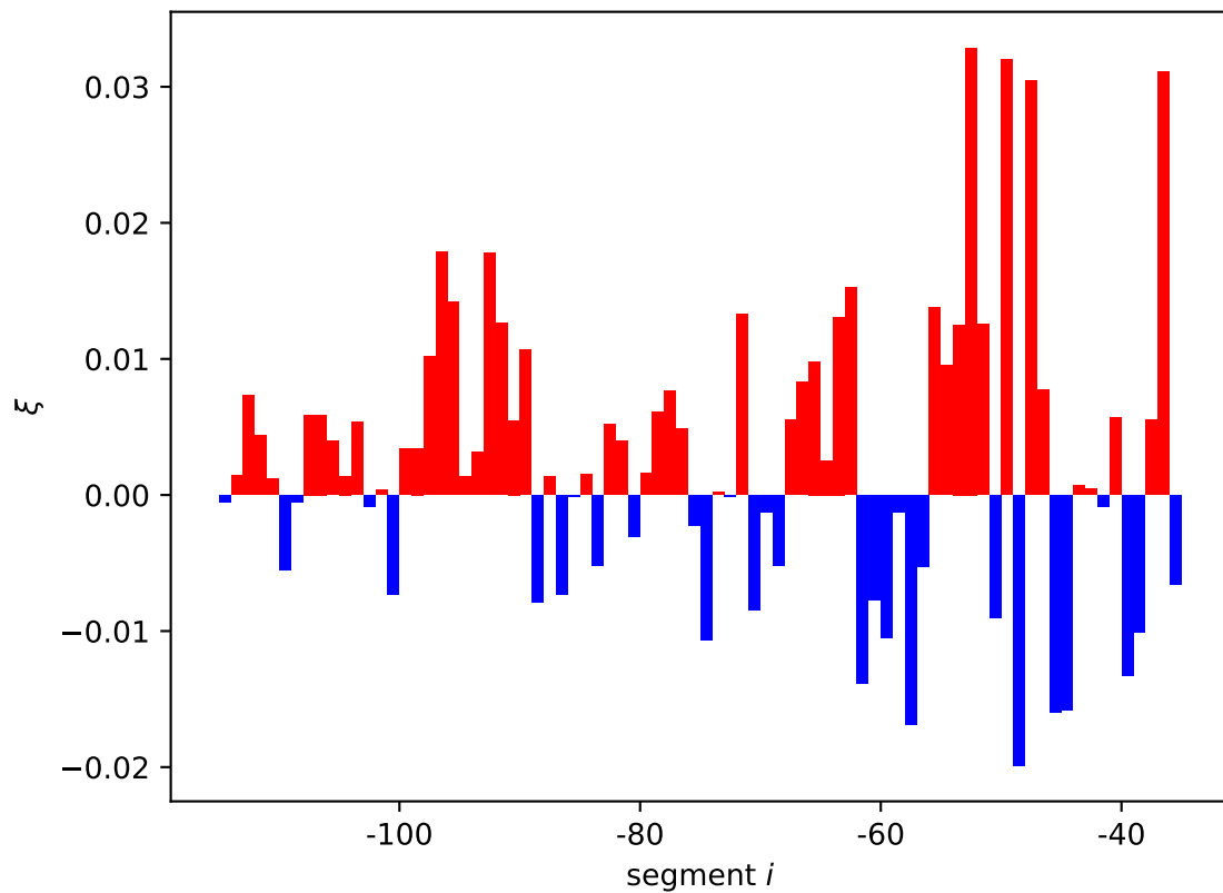
yedK expression shift \xi_i[01, 10]
