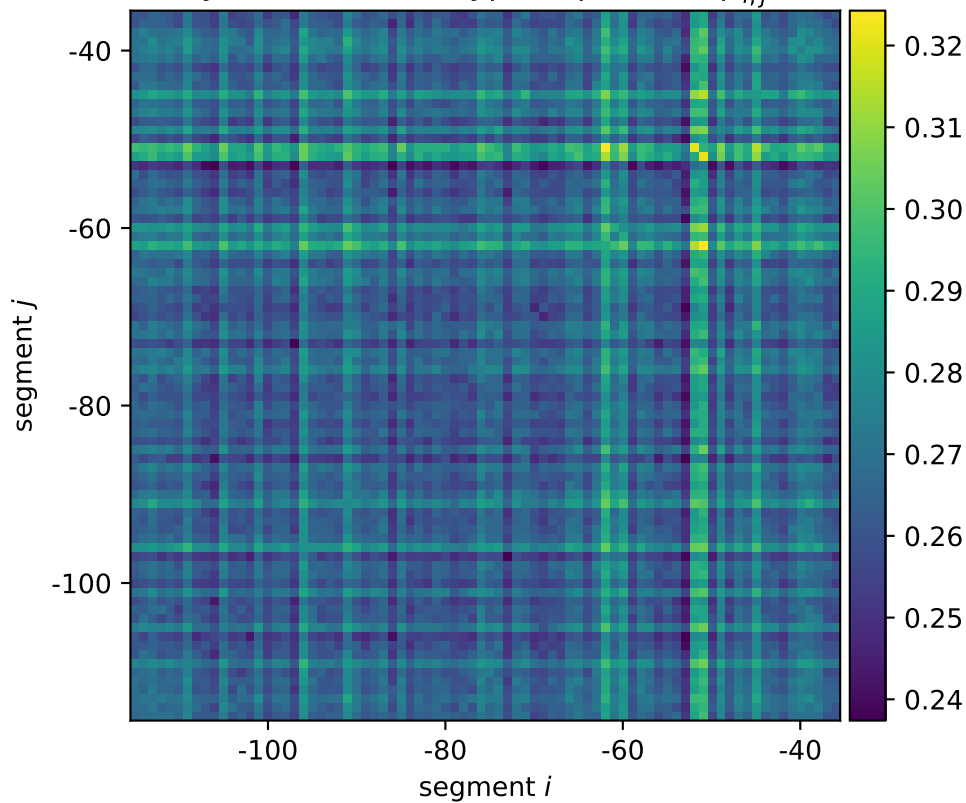
yedK mean wildtype expression \mu_{i,j}^*
