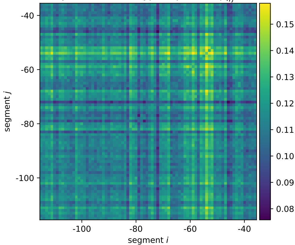
yehS mean wildtype expression \mu_{i,j}^*
