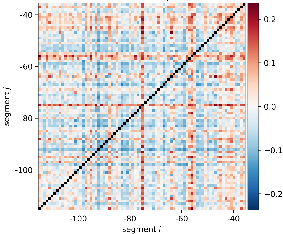
yehU expression shift \xi_{i,j}[\text{0011}, \text{1100}]
