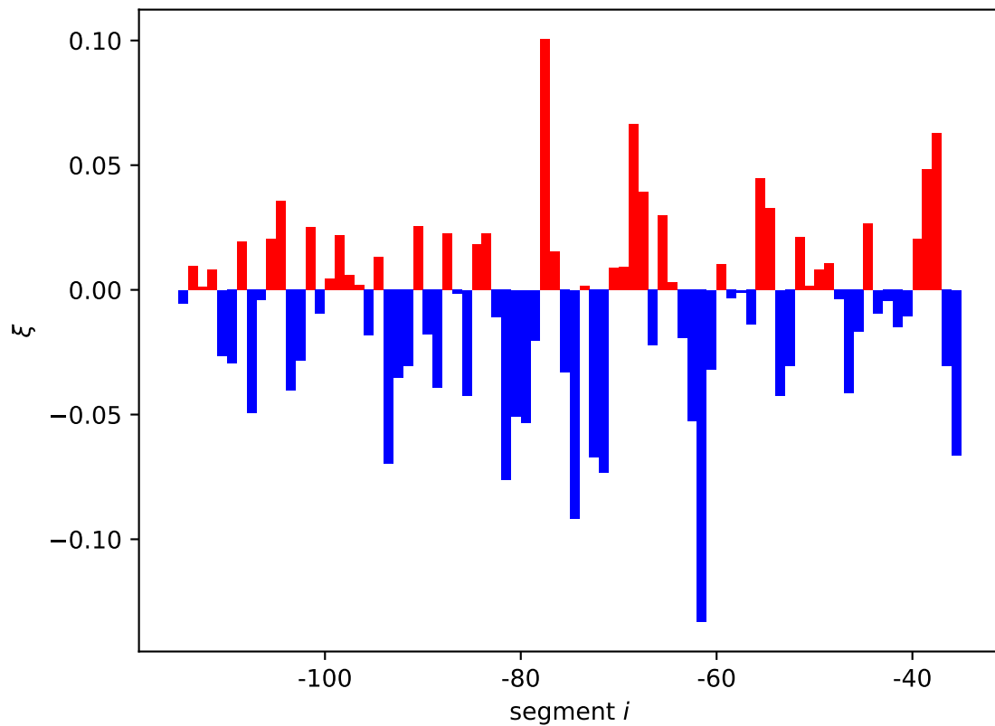
yehU expression shift \xi_i[01, 10]
