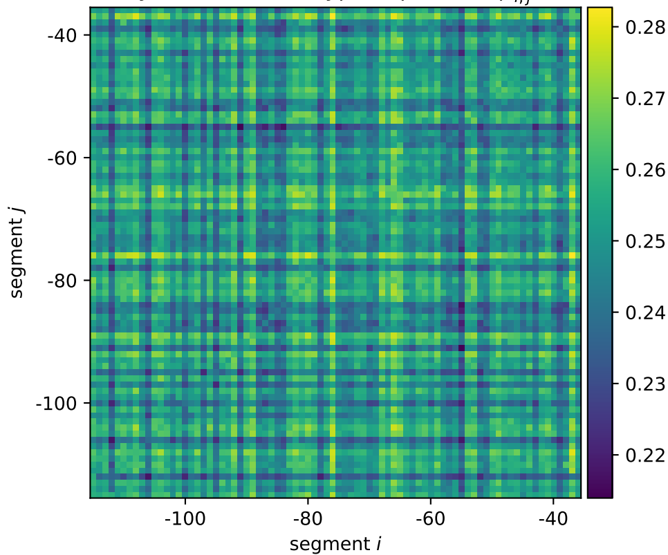
yehU mean wildtype expression \mu_{i,j}^*
