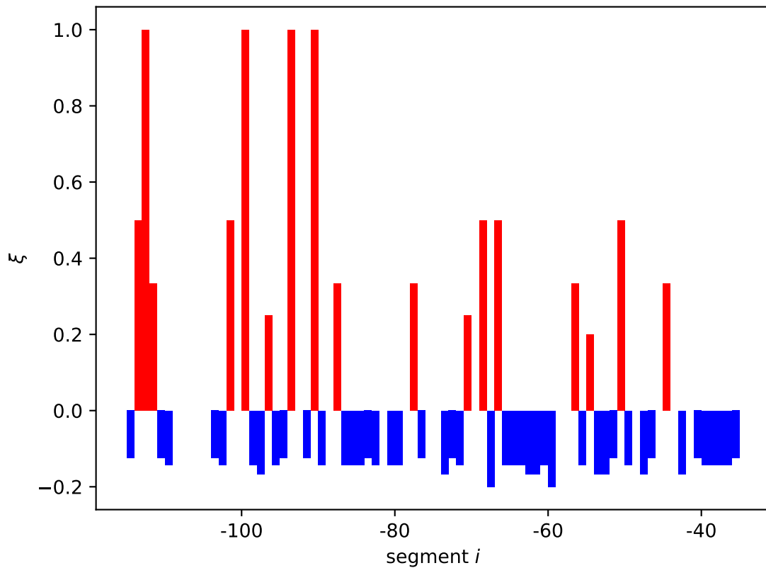
yehU expression shift \xi_i[01, 10]
