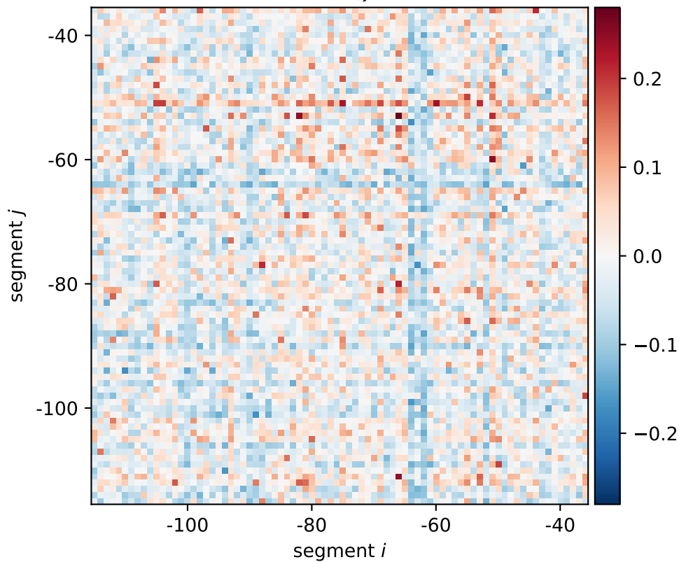
yeiQ expression shift \xi_{i,j}[0101, 0110, 1010]
