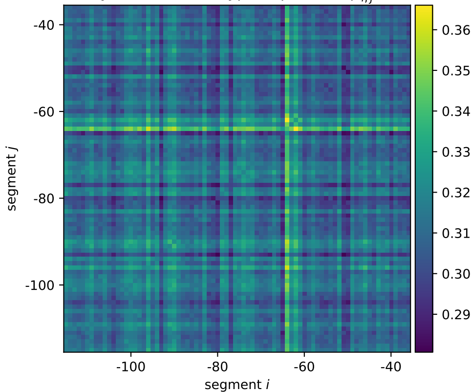
yeiQ mean wildtype expression \mu_{i,j}^*
