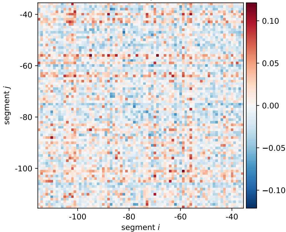
yfhG expression shift \xi_{i,j}[0101, 0110, 1010]
