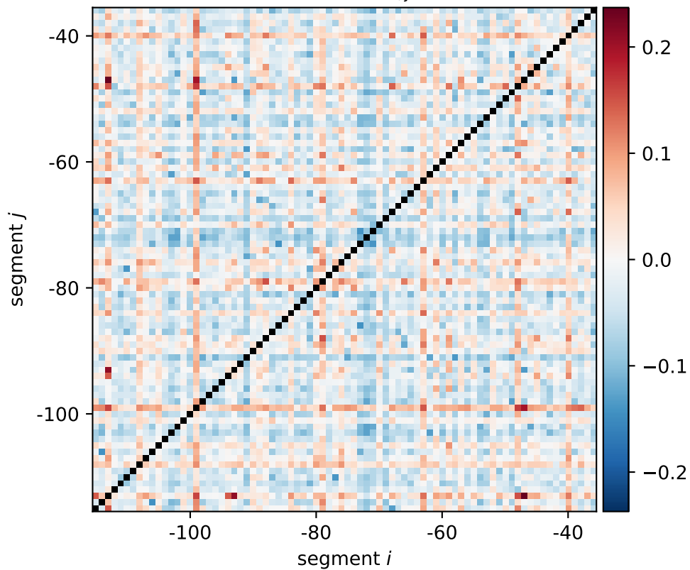
yfhG expression shift \xi_{i,j}[0011, 1100]
