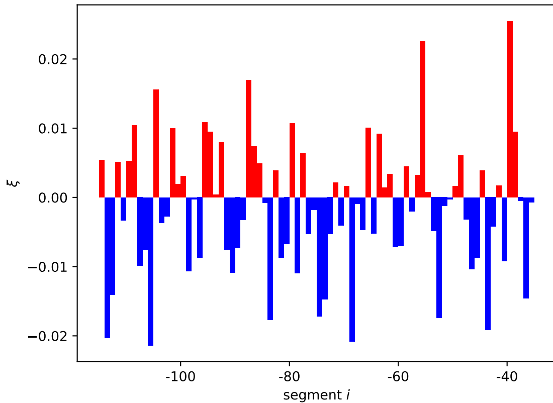
yfhG expression shift \xi_i[01, 10]
