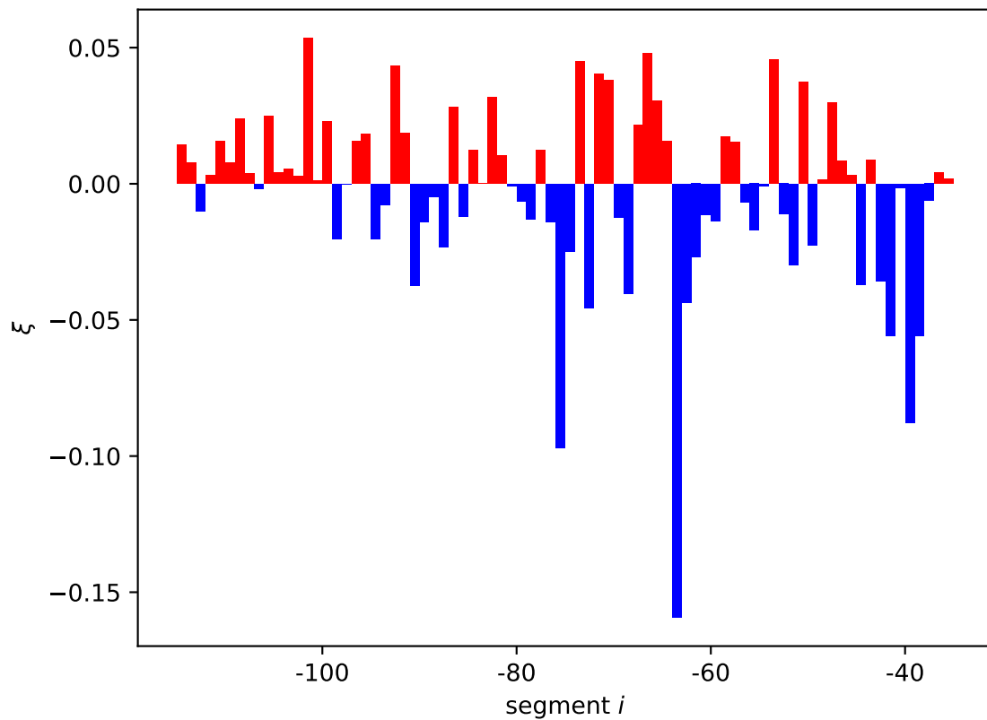
ygdH expression shift \xi_i[01, 10]
