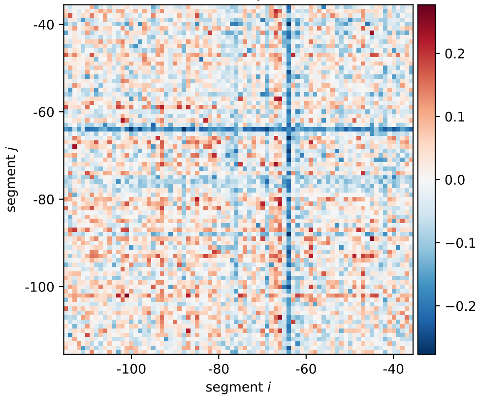
ygdH expression shift \xi_{i,j}[0101, 0110, 1010]
