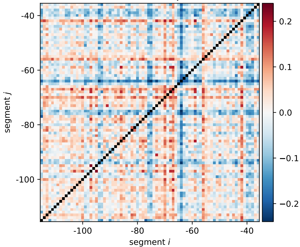
ygdH expression shift \xi_{i,j}[0011, 1100]
