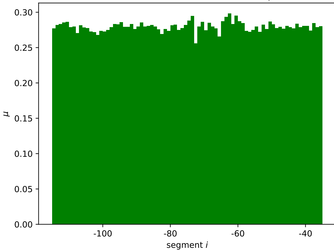
ygeR mean wildtype expression \mu_i^*
