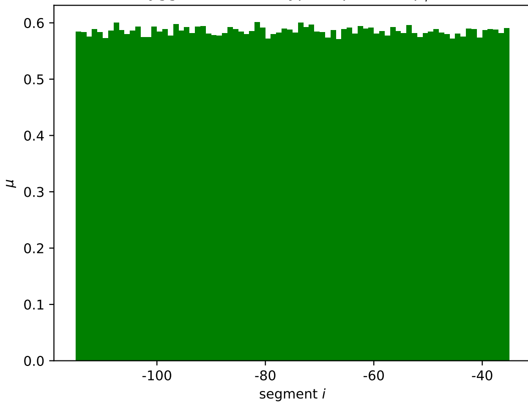
yggW mean wildtype expression \mu_i^*
