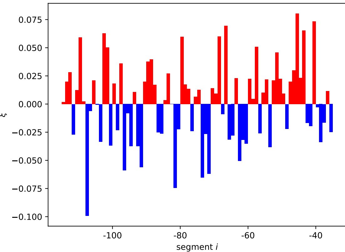
yggW expression shift \xi_i[01, 10]
