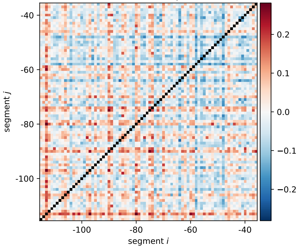
yggW expression shift \xi_{i,j}[\text{0011}, \text{1100}]
