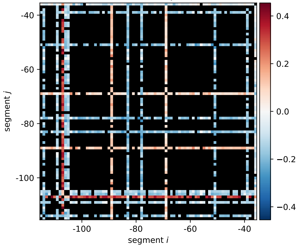
yicl expression shift \xi_{i,j}[0011, 1100]
