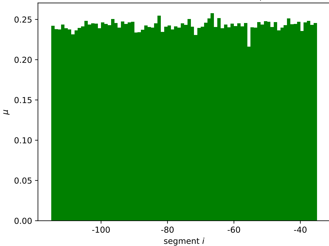
yicl mean wildtype expression \mu_i^*
